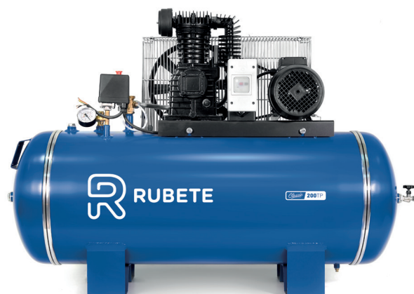
CLASSIC 200 TP
